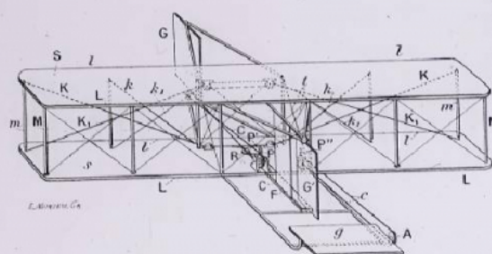
Fig. 1. - Aeroplanes Wright 1907.
