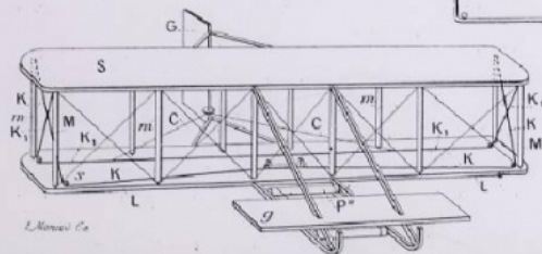
Fig. 3. - Aeroplano Wright 1905.
