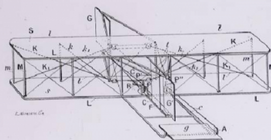
Fig. 1. — Aeroplane Wright 1907.
